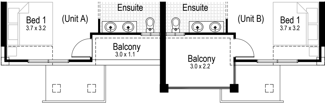
First Floor - Balcony Option
